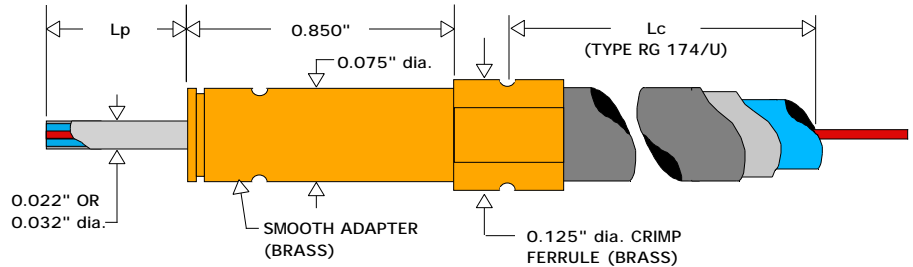
CA-1041 / 1208 SMOOTH BODY ADAPTER
