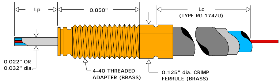
CA-1041 / 1208 THREADED BODY ADAPTER
