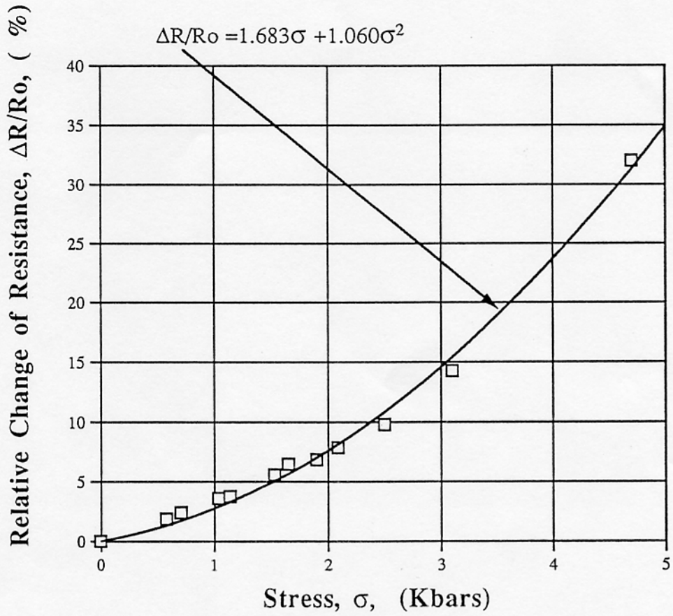
Plane Wave Calibration of Ytterbium Stress Gauge
